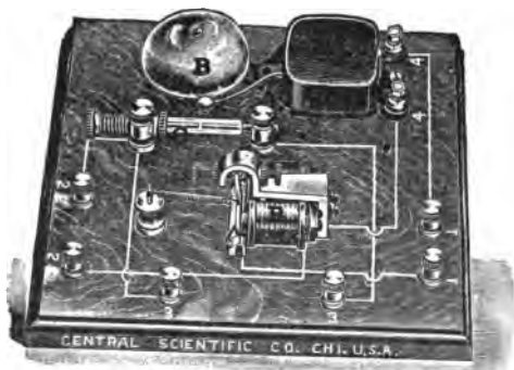
FIG. 59.—Receiver for Experimental Wireless Telegraph Set of Few Metres Range.
